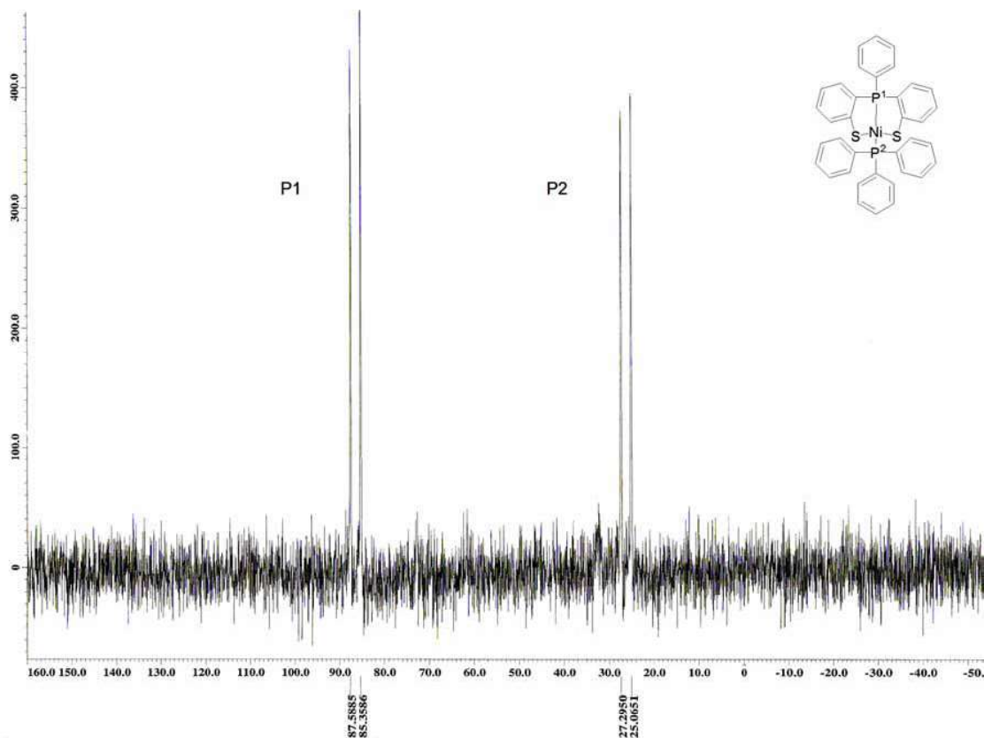
Figura 3.8 Espectro de RMN {}^{31}\text{P}\{^1\text{H}\} (121 MHz, \text{CDCl}_3 ) a 25°C del compuesto [\text{Ni}(\text{phPS}_2)(\text{PPh}_3)] (7).
